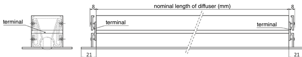
LONGITUDINAL VIEW OF DL DIFFUSER [with terminals]
